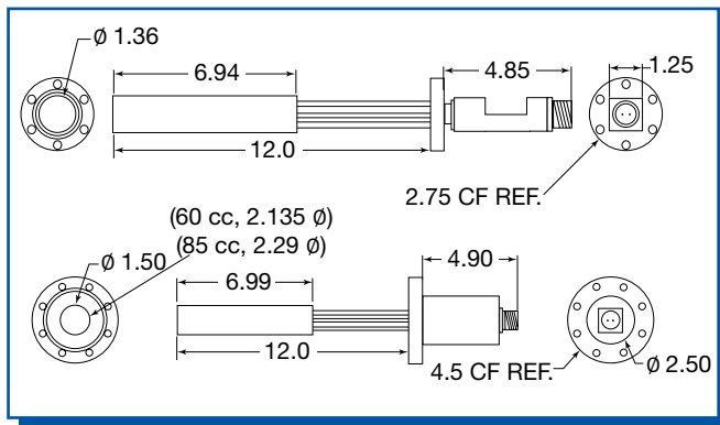
Schematic drawing of Hot-Lip Effusion Cells. Dimensions are given in Inches.
