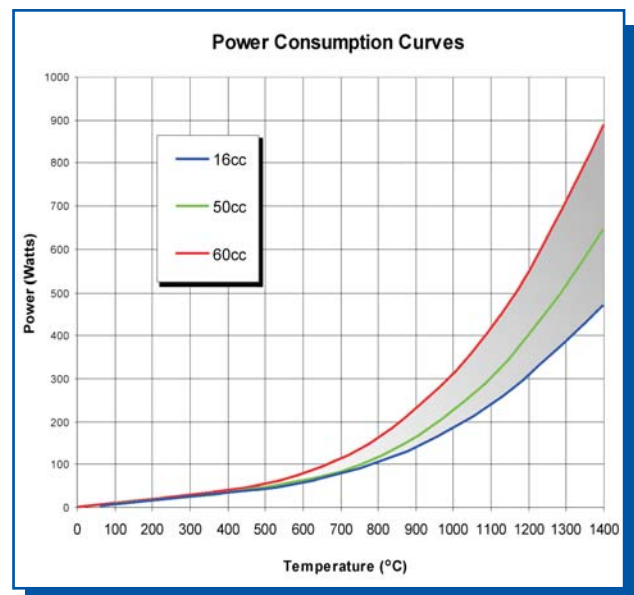
Typical power consumption of 16 cc – 60 cc Hot-Lip Cells.
