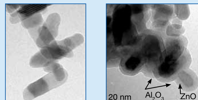
Before and after \text{Al}_2\text{O}_3 coating (~4 nm)
