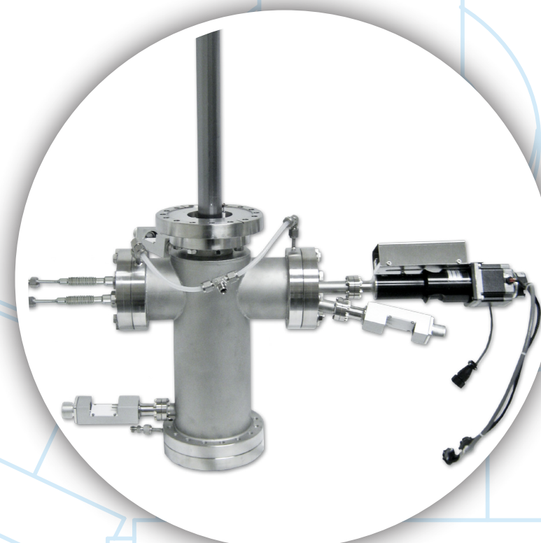
Valved Crackers
